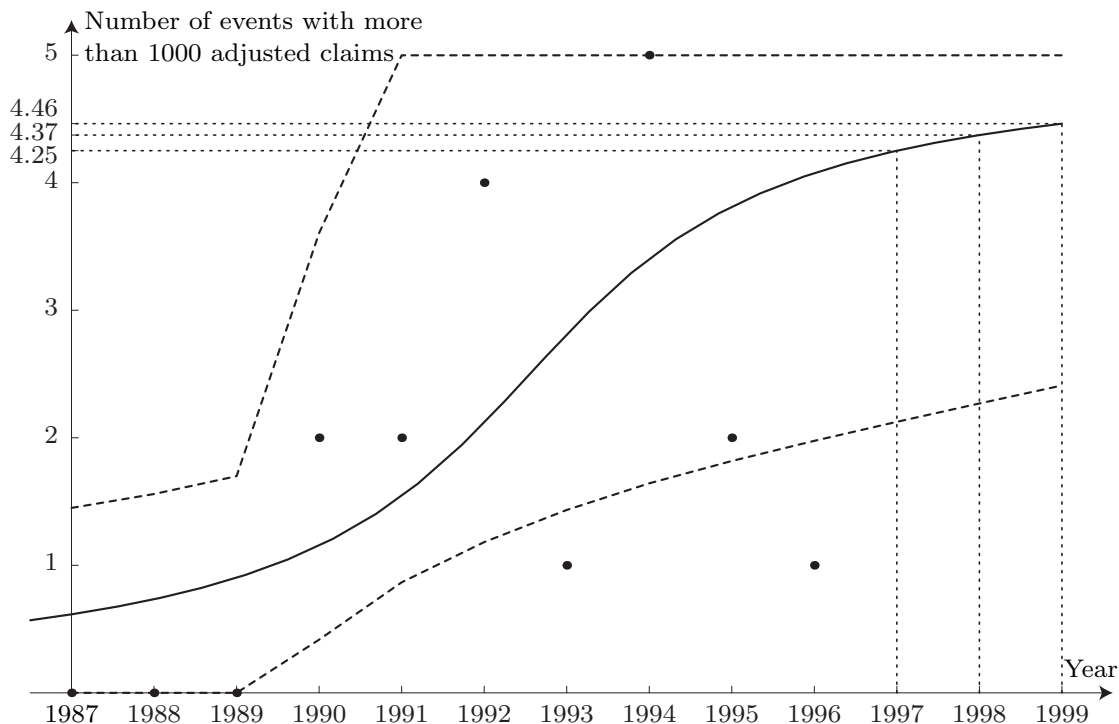
FIGURE 7.5. A smooth transition of the Poisson parameter according to (7.11). The possible range of the parameter is determined by the smallest and largest observed value, respectively. The maximum-likelihood method leads to \hat{\alpha} \approx -0.466 and \hat{\beta} \approx 0.442 . The dashed piecewise linear curves indicate the estimated 68%-confidence intervals for \lambda_{\hat{\alpha}, \hat{\beta}}(y) as derived from the log-likelihood ratio statistic. These intervals clearly show the artificial restriction of the range of the Poisson parameter.
