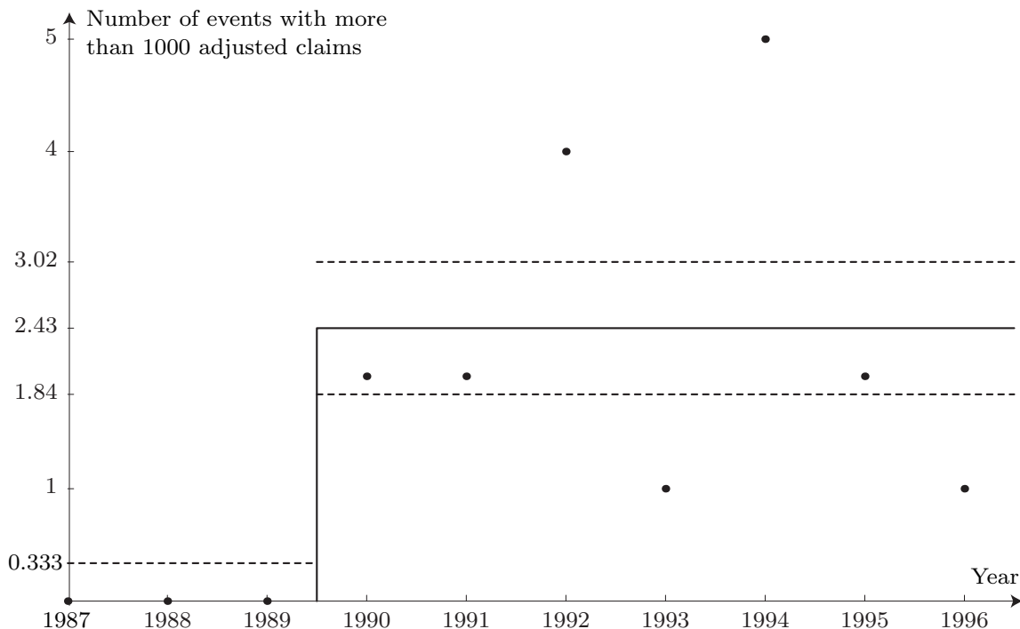
FIGURE 9.1. A model with a change-point in the Poisson parameter. A change from \lambda_0 = 0 to \lambda_1 = 17/7 \approx 2.43 between 1989 and 1990 maximises the likelihood. The dashed lines indicate the estimated standard deviations of the Poisson parameters disregarding the uncertainty arising from the estimate of the location of the change-point.
