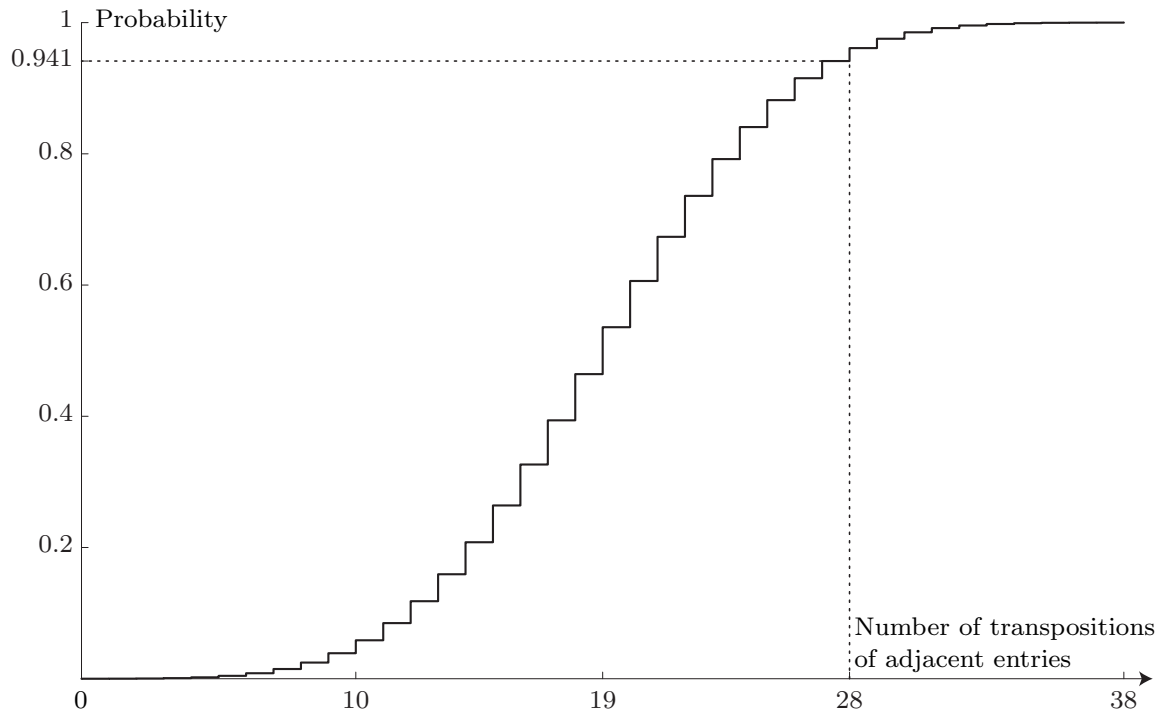
FIGURE 5.1. Distribution function of the number of successive transpositions of adjacent entries necessary to order a random permutation of the ten observations into decreasing order. For the observed data, 28 transpositions are necessary. At least 28 transpositions are necessary for about 5.86% of all permutations.
