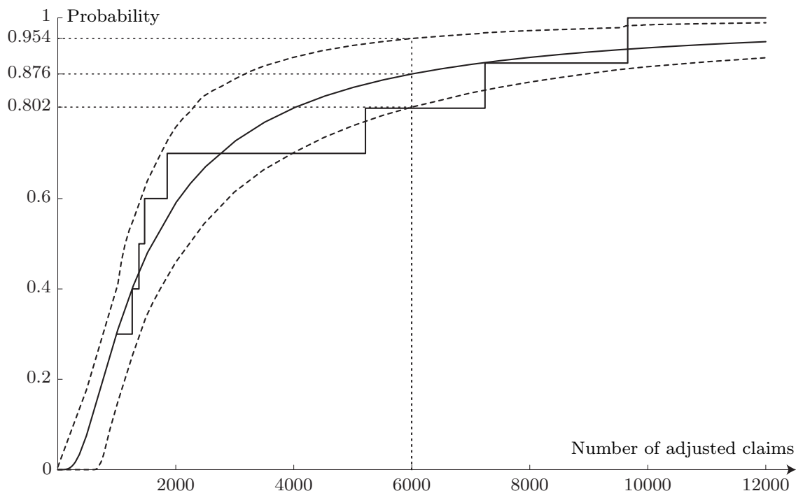
FIGURE 6.1. The censored empirical distribution function of the number of adjusted claims of the most severe event per year (solid step function) and the fitted generalised extreme value distribution (solid curve) with estimated exponent 1/\hat{\xi} \approx 1.316 , scale parameter \hat{\tau} \approx 1008 and location parameter \hat{\mu} \approx 1168 . The estimated probability, that no knock-out event occurs within one year, is approximately 0.876. The two dashed curves, derived from 1000 bootstrap samples, indicate 68%-confidence intervals for the fitted generalised extreme value distribution.
