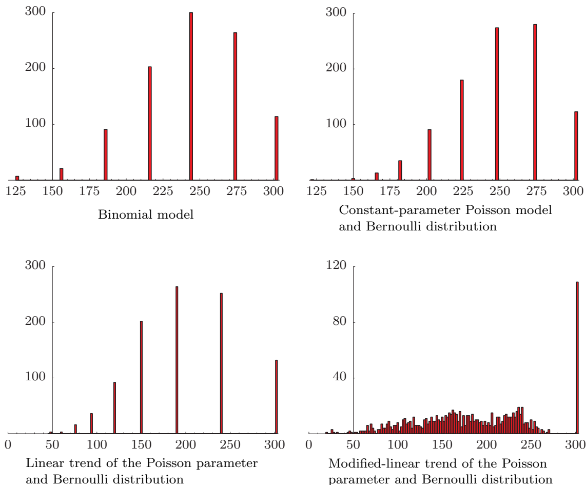
FIGURE 13.1. Distribution of the estimated coupon values for models no. 1, 4, 21, and 23 of Table 11.1 resulting from 1 000 simulated data sets. The mean, median, standard deviation and 15.9%-quantil are given in Table 12.1. Note the different scales, the discreteness of the two upper and the lower left distribution, the different sizes of the gaps, and the persistence of the peak at the highest possible coupon value representing the number of simulated data sets without a knock-out event.
