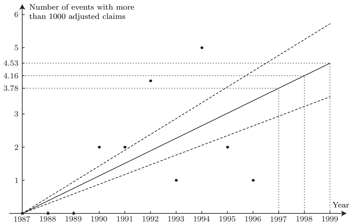
FIGURE 7.1. Observed number of events causing more than 1000 adjusted claims. A linear fit of the intensity \lambda_\beta(y) = \beta(y - 1987) , using the maximum-likelihood method, leads to \hat{\beta} = 17/45 \approx 0.378 . The increasing dashed lines indicate this estimated standard deviation of \lambda_{\hat{\beta}}(y) . This model has a problem with the years up to 1987 and it certainly underestimates the standard deviation in the first years.
